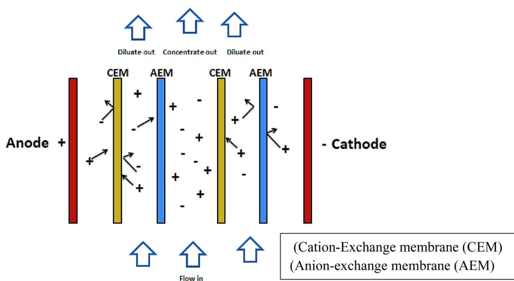
Fig. 14 Electrodialysis. 139
