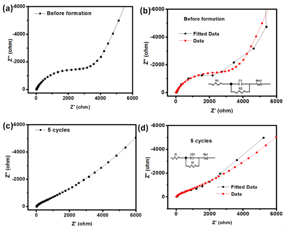
Fig. 13 EIS spectra of the Si–Gr@Gr anode with the crosslinked CMC–PAA binder (a) before formation, (b) fitted data before formation, (c) after 5 cycles and (d) fitted data after 5 cycles.
