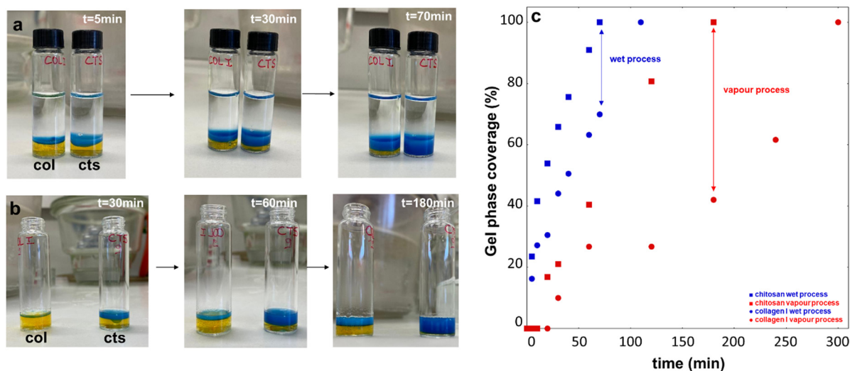
Fig. 7 Study of the kinetics of gelation. Visual evolution in the presence of bromothymol blue of collagen (col) and chitosan (cts) solutions at 25 mg mL -1 (a) mixed with ammonia and (b) under ammonia vapours. (c) Evolution of sol-gel coverage for both solutions and both gelation routes.
