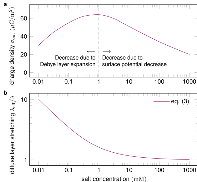
Fig. 5 (a) Surface charge density as a function of salt concentration (exemplary values), with proposed physical mechanisms for the trends. Charge separation first increases with salt concentration and then decreases. (b) For a given velocity of the order of 10 \text{ cm s}^{-1} , the expansion of the diffuse layer is strongest for low salt concentrations and diminishes at high concentrations. Trend line calculated with eqn (3).
