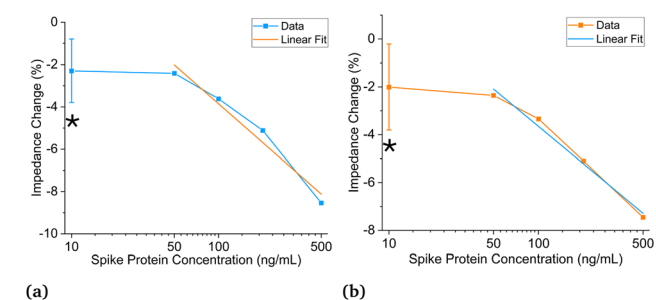
Fig. 4 Sensing of spike protein in saliva with antibody in 1 \times PBS solution. (a) Titration curve using updated data analysis method for SARS-CoV-2 spike proteins in saliva and antibodies in 1 \times PBS with 50–500 \text{ng mL}^{-1} dynamic range and 200 \text{ng mL}^{-1} (1.5 nM) detection limit; linear fit: (Z) = 8.36 - 6.11 \times (C) , R -square = 0.97. (b) Titration curve using previous data analysis method for SARS-CoV-2 spike proteins in saliva and antibodies in 1 \times PBS with 50–500 \text{ng mL}^{-1} dynamic range and 200 \text{ng mL}^{-1} (1.5 nM) detection limit; linear fit: (Z) = 6.74 - 5.2 \times (C) , R -square = 0.99. * Denotes negative control ( C = 0 \text{ ng mL}^{-1} ) plotted at C = 10 \text{ ng mL}^{-1} for visualization purposes, N = 5 for C = 0 \text{ ng mL}^{-1} , N = 1 for all other concentrations.
