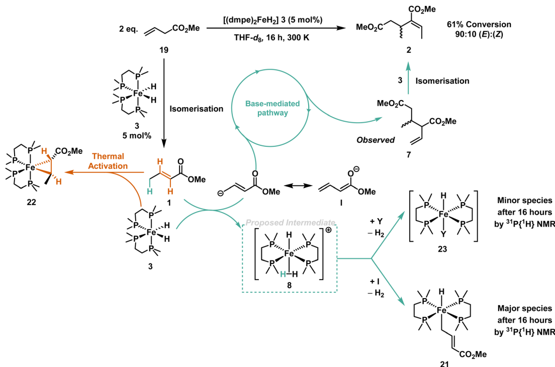
Scheme 2 Isomerisation of methyl 3-butenate 19 to methyl crotonate 1 by [(dmpe) 2 FeH 2 ] 3 . Methyl crotonate 1 can then be dimerised by the base-mediated pathway to give the dimer intermediate dimethyl 2-ethenyl-3-methylpentanedioate 7 which itself can be isomerised by [(dmpe) 2 FeH 2 ] 3 to give ( E ),( Z )-2-ethylidene-3-methylpentanedioate 2 . 31 P NMR spectroscopic analysis of the reaction shows that the major iron species is trans -[(dmpe) 2 FeH(CH 2 CH=CHCO 2 Me)] 21 , with minor amounts of [(dmpe) 2 FeHY] 23 . Minor amounts of [(dmpe) 2 Fe(η 2 -1)] 22 by thermal activation of [(dmpe) 2 FeH 2 ] 3 were also observed.
