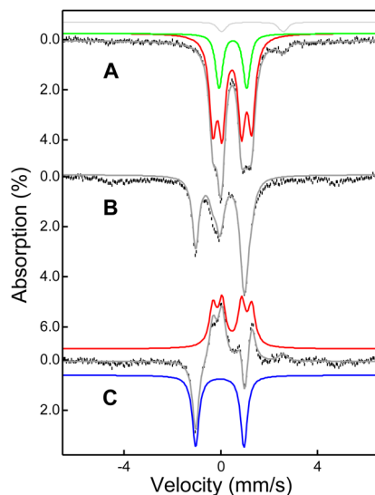
Fig. 4 4.2 K zero field Mössbauer spectra (vertical bars) of 2+\text{Sc} (panel A) and upon conversion of 2+\text{Sc} into 3 (panel B). Panel C shows the B - A difference spectrum highlighting the conversion of 2+\text{Sc} to 3 . Panel A shows an overall simulation (grey solid line) with four species. The red solid line containing two distinct ferric doublets of equal intensity represents 74% of the iron in the sample and is assigned to the dominant 2+\text{Sc} species with distinct \text{Fe}^{\text{III}} units. The green solid line represents 18% of the iron in the sample corresponding to a symmetric diferric species. The light grey line represents a minor ferrous species (~5%), likely to be the starting ferrous complex. Panel B shows an overall simulation (grey solid line) with 50% 3 , 25% 2+\text{Sc} and 18% 2' . Panel C shows the conversion of 2+\text{Sc} (red solid line) into 3 (blue solid line).
