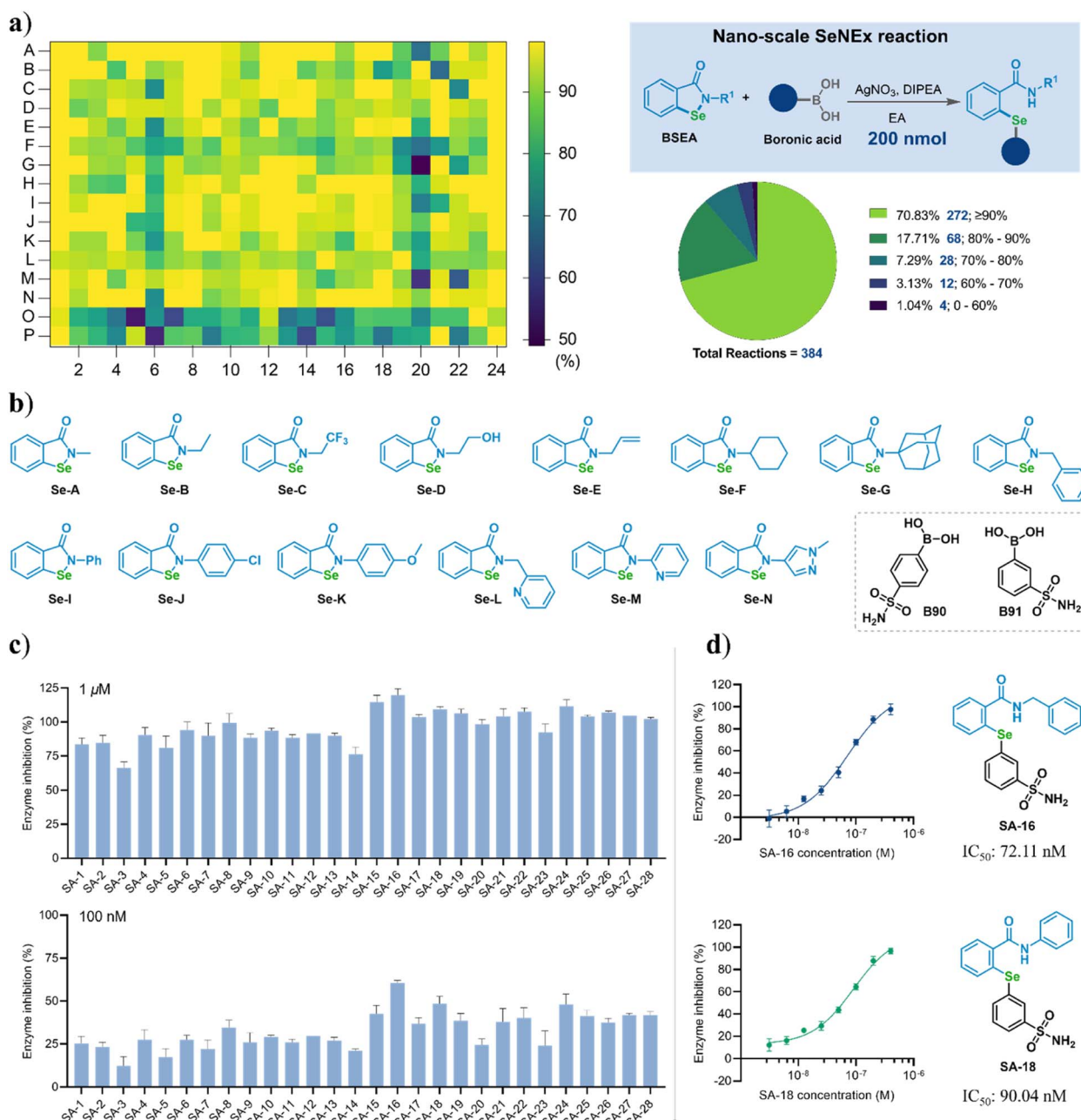
Fig. 5 On-microplate nanomole-scale parallel synthesis enables efficient identification of novel CA XII inhibitors. (a) 16 \times 24 nanomole-scale parallel synthesis on 96-well microplates. (b) 14 \times 2 nanomole-scale parallel synthesis on 96-well microplates. (c) Inhibitory rates of 28 compounds against CA XII at 1 \mu\text{M} and 100 nM. (d) \text{IC}_{50} determination of SA-16 and SA-18; each experiment was run three times independently ( n = 3 ). Standard condition of parallel synthesis: BSEAs (200 nmol), boronic acids (200 nmol), DIPEA (300 nmol), and \text{AgNO}_3 (5 mol%) in EA (50 \mu\text{L} ), 50 ^\circ\text{C} , and 6 h (without air exclusion). Conversions are determined by LC-MS analysis. LC-MS, liquid chromatography-mass spectrometry.
