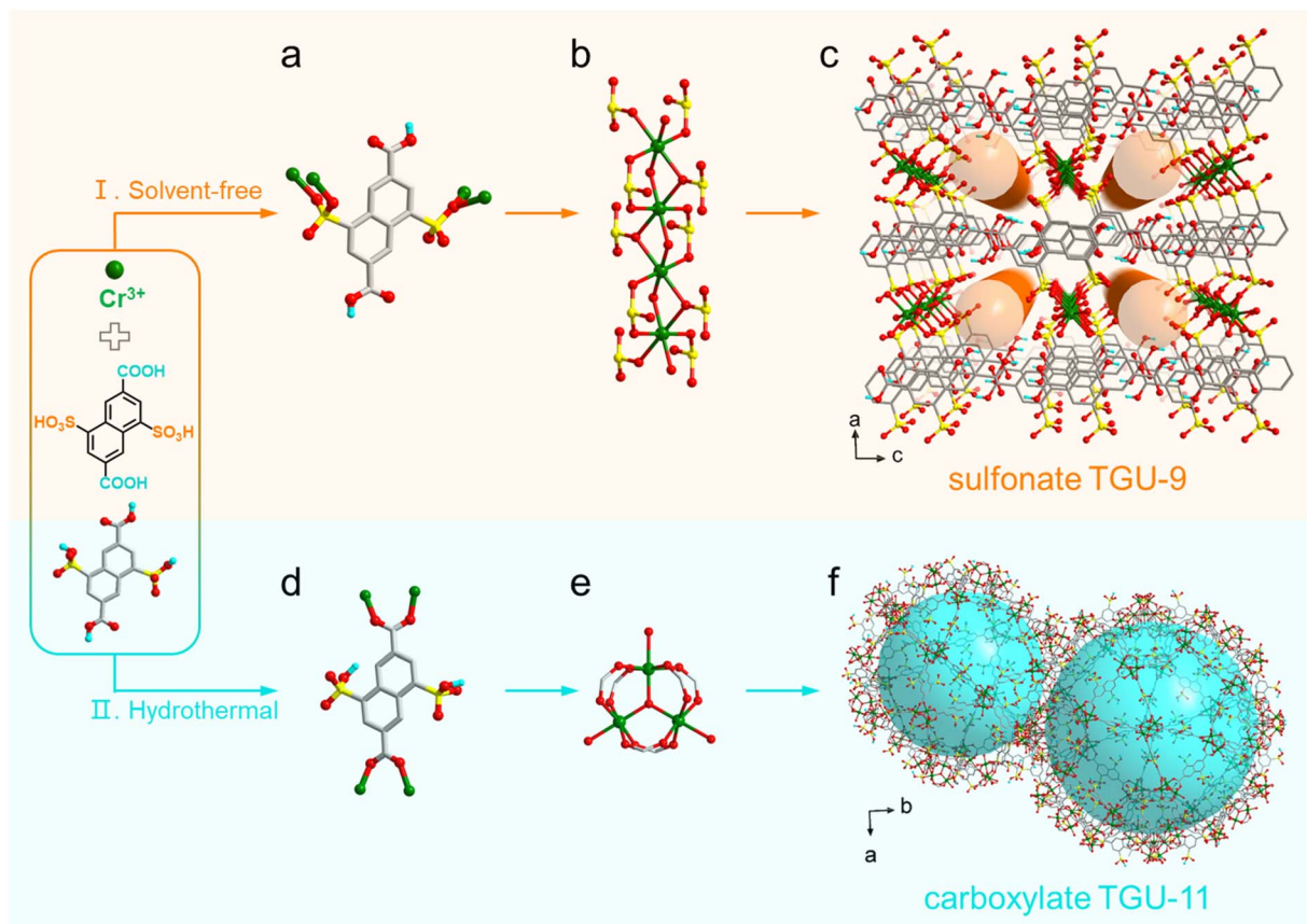
Fig. 2 Reversed coordination preference: from Cr-carboxylate coordination in aqueous solution to Cr-sulfonate coordination under solvent-free conditions. (a) Sulfonate coordinated NAP(COOH) 2 (SO 3 H) 2 2- linker with four Cr 3+ ions. (b) 1D Cr-SO 3 SBU in TGU-9. (c) Sulfonate TGU-9 viewed along the b axis. (d) Carboxylate coordinated NAP(COO) 2 (SO 3 H) 2 2- linker with Cr 3+ ions. (e) Cr 3 trimer. (f) Carboxylate TGU-11 viewed along the c axis. H atoms are omitted for clarity, except those on acid groups.
