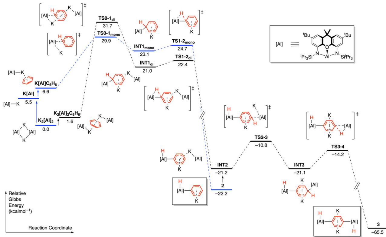
Fig. 3 Gibbs free energy profile (PBE0-D3 BJ -CPCM(benzene)/Def2-TZVPP//PBE0-D3 BJ /BS1) for the reaction between the transiently generated K_n[\text{Al}(\text{TIPSON})]_n ( n = 1, 2 ) alumanyl complex and benzene to give C–H activation complexes 2 and 3 . Relative Gibbs free energies are presented in kcal mol -1 . Monomeric pathway highlighted in blue.
