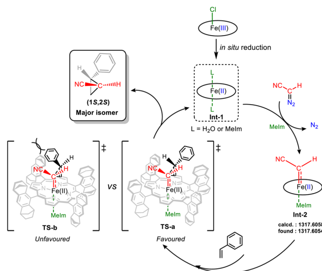
Scheme 8 Plausible mechanism of (+)\text{-D}_4\text{-(por)FeCl} -catalyzed asymmetric cyclopropanation.
