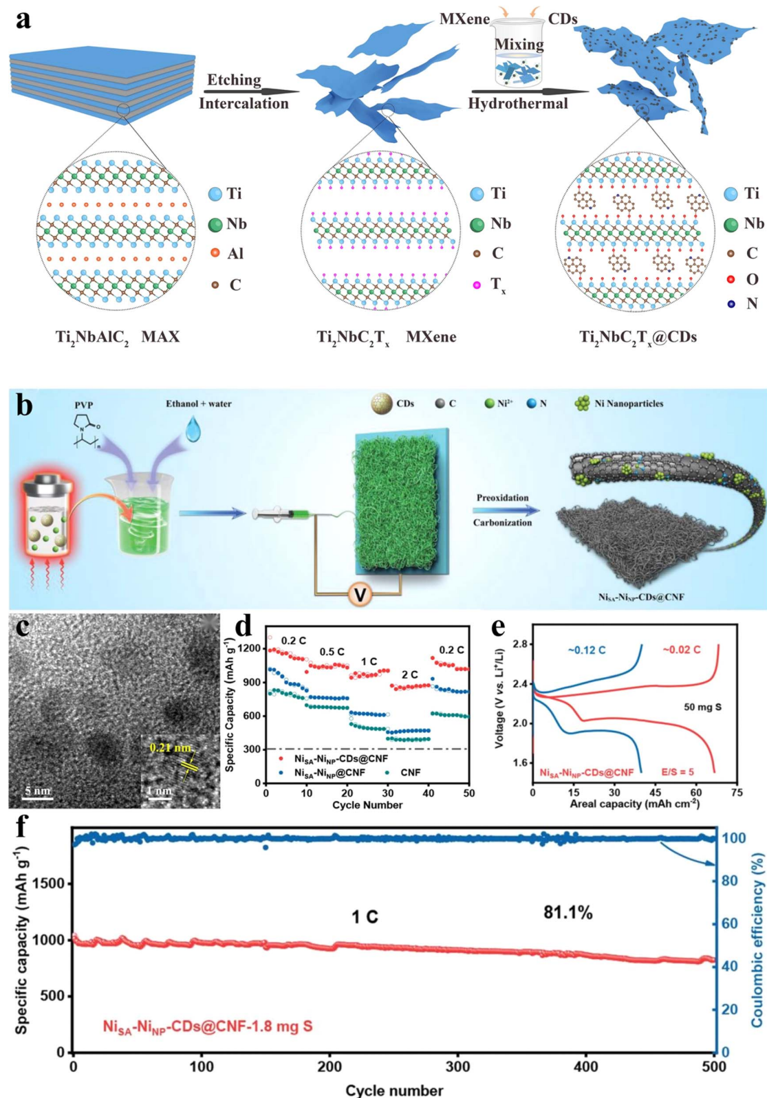
Fig. 6 Application of BCDs in lithium batteries: (a) a schematic diagram of the edge-crumpled Ti_2NbC_2T_x@CDs nanosheets; (b) schematic depiction of Ni_{SA-NiNP-CDs@CNF} ; (c) TEM image of as-produced CDs of the Ti_2NbC_2T_x@CDs composite ((inset): HRTEM image of the CDs); (d) rate performance of different cathodes; (e) charge-discharge curves and (f) cycling stability of a sulfur cathode (sulfur loadings: 50 mg cm^{-2} and E/S = 5 \mu L mg^{-1} ). (a and c) Reproduced with permission. 96 Copyright 2024, Elsevier. (b, d–f) Reproduced with permission. 97 Copyright 2022, Wiley-VCH.
