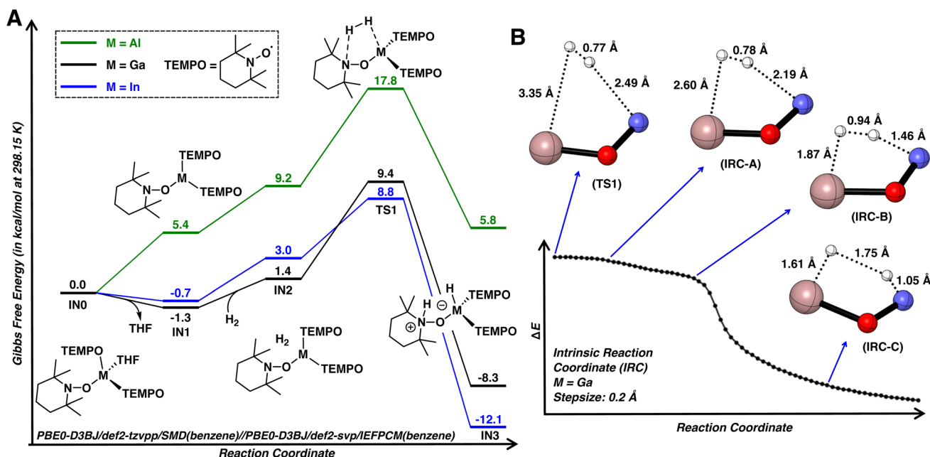
Fig. 5 (A) Computed reaction pathway for H_2 activation by complexes 1 ·THF, 2 ·THF, and 3 ·THF. (B) Forward intrinsic reaction coordinate for TS1 ( M = Ga ) and associated bond lengths of selected structures. Selected atoms were omitted for clarity. Color code: N, blue; O, red; Ga, salmon; H, white.
