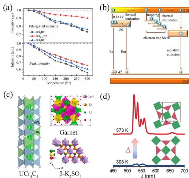
Fig. 5 (a) The emission retention of peak intensity and integrated intensity of \text{K}_x\text{BP}:\text{Eu}^{2+} ( x = 0, 1.25, 2 ) as a function of temperature and (b) a suggested model for describing the mechanism of improved thermal stability. Reproduced with permission from ref. 135. Copyright 2022, Elsevier. (c) \text{UCr}_4\text{C}_4 structure, garnet structure, and \beta\text{-K}_2\text{SO}_4 structure model. 142–144 Reproduced with permission from ref. 142–144. Copyright 2023, ACS. Copyright 2023, Elsevier. Copyright 2018, ACS. (d) Thermal enhancement in \text{Er}^{3+} -doped orthorhombic \text{Yb}_2\text{W}_3\text{O}_{12} by negative thermal expansion. Reproduced with permission from ref. 145. Copyright 2023, WILEY-VCH.
