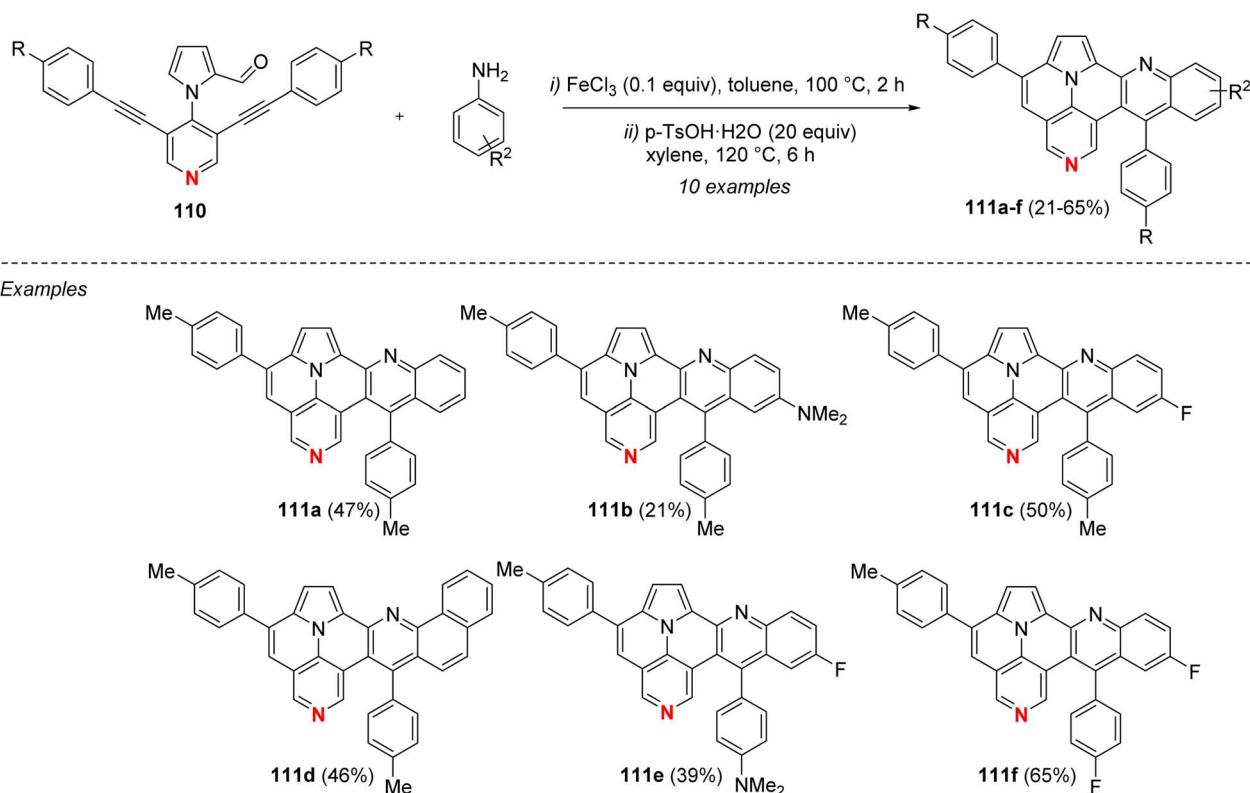
Scheme 29 Synthesis of quinolino-aza-ullazines 111a–f .
