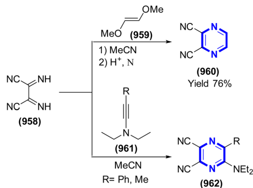
Scheme 266 Synthesis of pyrazine.
