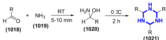
Scheme 283 Synthesis of 2,4,6-trialkyl-1,3,5-hexahydrotriazine.
