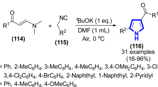
Scheme 32 Synthesis of 2,4-disubstituted pyrroles catalyzed by t\text{BuOK} .
