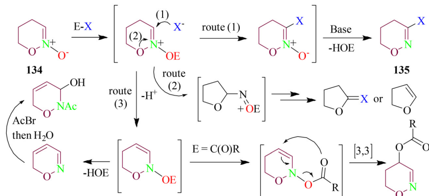
Scheme 54 Nucleophilic halogenation of cyclic nitronates.
