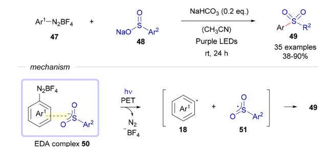
Scheme 7 Sulfonylation transformations of aryl diazonium salts 47 via light-driven excitation of EDA complexes 50 .
