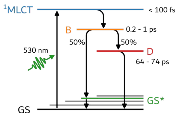
Figure 8. Proposed relaxation scheme for the family of complexes. The ^1\text{MLCT} is populated and depleted within less than 100 fs. Its depopulation corresponds to the population of state B that decays over the ps timescale into a hot ground state \text{GS}^* and the long-living state D .
