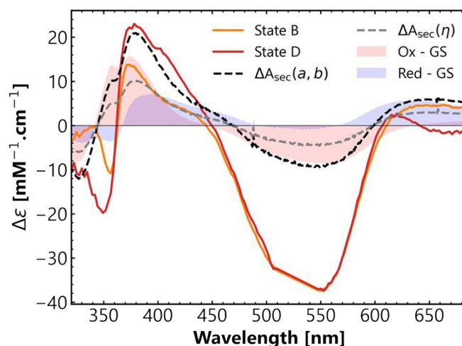
Figure 9. Difference absorption spectra of complex fac-C2 in oxidised-minus-ground state (red) and reduced-minus-ground state (blue) forms. The solid lines correspond to the species-associated difference spectra of states B and D (SADS, orange and red). Dashed lines refer to simulations of the differential spectrum of an MLCT-equivalent state, computed either by the approach of ref. 26 (grey dashed) or by the formulas developed in section 6 of the Supp. Info. (black dashed line). Note that \alpha_{\text{red}} = \alpha_{\text{ox}} = 1 was used for the latter.
