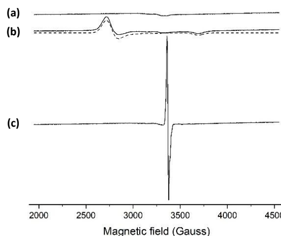
Figure 4. X-band cw-EPR spectra recorded at 100 K of a MeCN solution of fac - C2 (0.2 mM) containing 0.1 M TBAPF 6 . a) initial Fe(II) complex, b) after exhaustive electrolysis at E_{app} = 1.2 V vs SCE. Simulation in dashed line for a low-spin S = 1/2 Fe(III) complex with g_{\perp} = 2.452 and g_{\parallel} = 1.823 , c) after exhaustive electrolysis at E_{app} = -1 V vs SCE to generate an Fe(II)L • radical with g = 1.999 .
