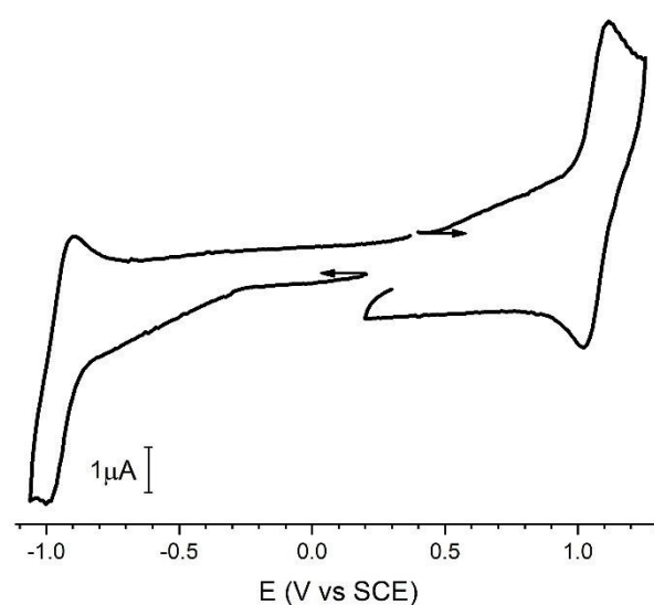
Figure 2. Cyclic voltammogram of fac-C2 (0.2 mM) in a MeCN solution containing 0.1 M TBAPF 6 , recorded at v = 100 \text{ mVs}^{-1} .
