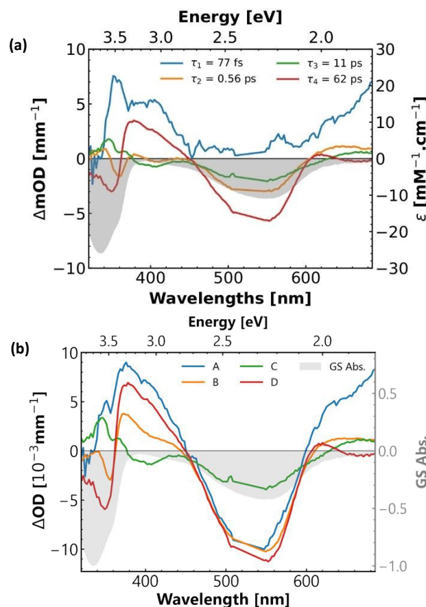
Figure 6. Decay-associated differential spectra of fac-C2 (a) from global analysis and species-associated spectra (b) of the same complex obtained with the relaxation scheme of Figure 8.
