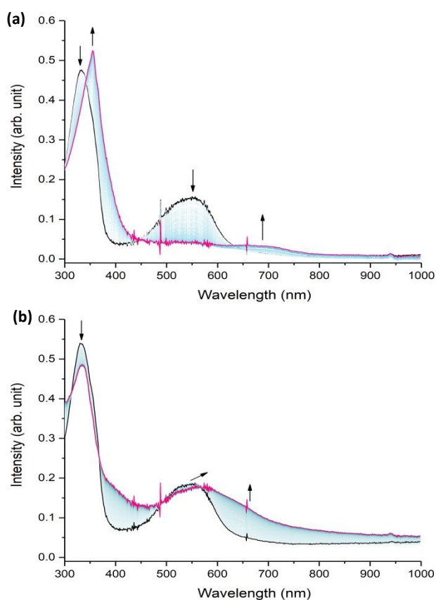
Figure 3. In situ UV-VIS spectra of fac - C2 (0.2 mM) in an acetonitrile solution containing 0.1 M TBAPF 6 , a) during exhaustive oxidation at E_{app} = 1.2 V vs SCE (last scan after 285 s), b) during exhaustive reduction at E_{app} = -1 V vs SCE (last scan after 570 s). (Pathlength of 1 mm and scan delay of 5 s between two spectra).
