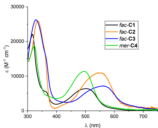
Figure 1. UV-VIS spectra of the complexes in acetonitrile solutions.
