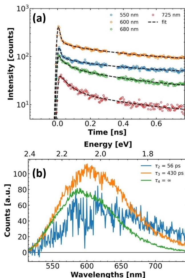
Figure 10. Time-resolved emission data of fac-C2 recorded with a streak camera (10 ps time resolution FWHM). Excitation with 0.3 ps pulses at 515 nm, and detection through a long-pass OG550 filter. (a) Kinetic traces of the time-dependent luminescence measurement with best fits as dashed lines. (b) Decay-associated spectra (DAS) of the different lifetimes found by global analysis.
