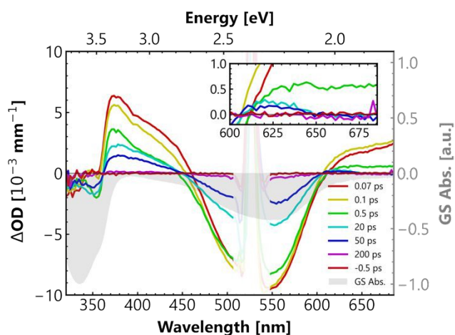
Figure 5. Selected differential transient absorption spectra of complex fac-C2 . Excitation wavelength 530 nm. The sign-inverted and arbitrarily scaled ground state absorption is plotted for comparison (grey). Inset: Zoom into the 600–700 nm region highlighting the narrowing of the red ESA between 0.5 and 20 ps delay.
