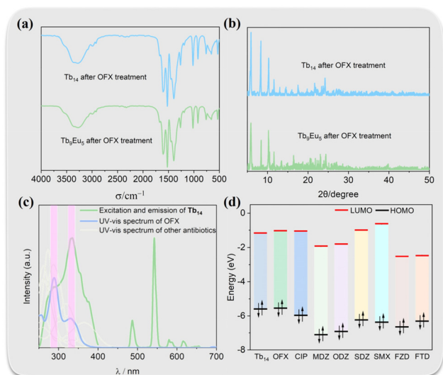
Fig. 7 (a) Infrared spectrum (b) and PXRD patterns of Tb_{14} after OFX treatment; (c) UV-vis absorption spectrum of antibiotics ( C = 10^{-5} M) and excitation and emission spectra of Tb_{14} in water suspension; (d) HOMO and LUMO energies and isosurfaces for Tb_{14} and antibiotics.
