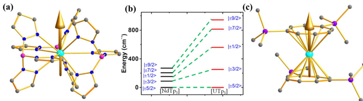
Fig. 4 (a) The magnetic anisotropy axis of [UTp_3] ( 1 ). (b) A comparison of CF splitting of five ground KDs of 1 and 2 . (c) The magnetic anisotropy axis of [\text{Li}(\text{DME})_3][\text{U}(\text{COT}'')_2] ( 3 ). Colour code: U (cyan), N (blue), Si (violet), B (pink), p (green) and C (grey). Hydrogens are omitted for clarity.
