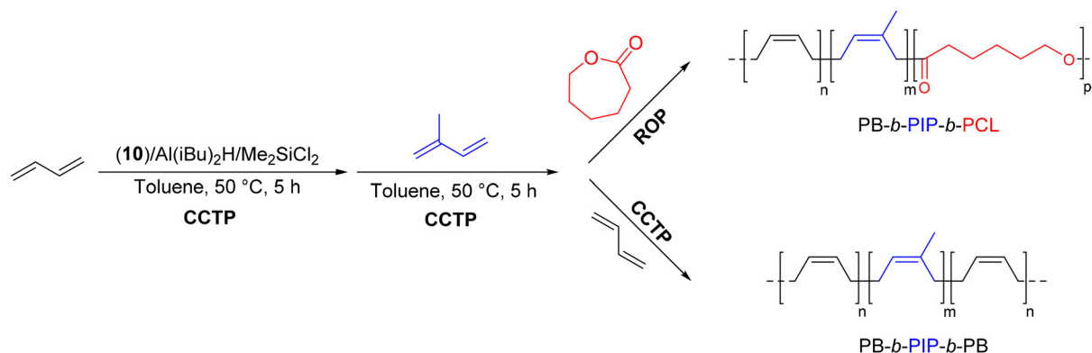
Scheme 28 Synthesis of PB- b -PIP- b -PB and PB- b -PIP- b -PCL triblock copolymers by CCTP and ROP with the Nd(OiPr) 3 /Al( i Bu) 2 H/Me 2 SiCl 2 catalytic system, step 1: [BD]/[Nd] = 500, step 2: [IP]/[Nd] = 500, and step 3: [BD]/[Nd] = 500/[ \epsilon -CL]/[Nd] = 300. 51
