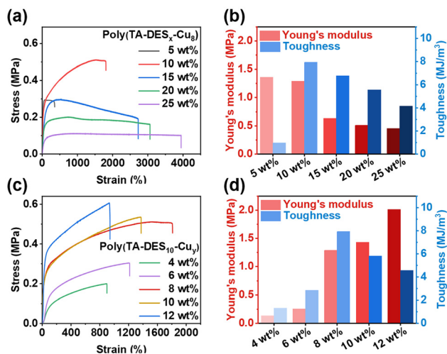
Fig. 2 (a) Tensile stress-strain curves of the resulting Poly(TA-DES x -Cu 8 ) with different weight ratios of DES ( x = 5, 10, 15, 20 and 25, respectively). (b) Young's modulus and toughness calculated from the tensile stress-strain curve of Poly(TA-DES x -Cu 8 ). (c) Tensile stress-strain curves of the resulting Poly(TA-DES 10 -Cu y ) with different weight ratios of Cu 2+ ( y = 4, 6, 8, 10 and 12, respectively). (d) Young's modulus and toughness calculated from the tensile stress-strain curve of Poly(TA-DES 10 -Cu y ).
