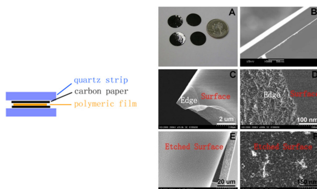
Fig. 5 Left: Sandwich-type-carbonization. Right: Photograph (A) and cross-sectional SEM image (B) of the OMC film. SEM images of as-made (C and D) and surface-etched (E and F) OMC. Reproduced from ref. 35 with permission from Elsevier, copyright 2025.
