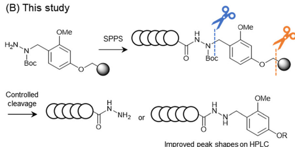
Fig. 1 Various methods for preparing peptide hydrazides.
