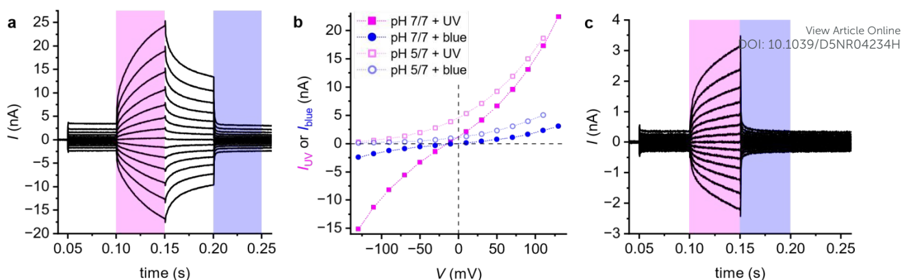
Figure 4: The transmembrane flux of the anionic protonophore CCCP^- is rapidly modulated by photoisomerization of membrane-embedded photolipids. a , Voltage-clamp current recordings on a photoswitchable PLB with 10 \mu M CCCP added to the aqueous compartments (100 mM KCl, 20 mM HEPES pH 7.0) on both sides. The recordings were made as in Figure 2b. As with valinomycin- K^+ , I increases upon UV light exposure and blue light reverts this increment. That is, the flux of CCCP^- is increased across the cis state membrane. b , I - V curves constructed as described in Figure 2c for recordings under symmetric (pH 7 at both sides; closed symbols) and asymmetric conditions (pH 5 at side 1, pH 7 at side 2; open symbols). Upon creating the gradient in pH by the addition of HCl to compartment 1, V_r shifted towards large negative values, consistent with proton-selective transport. Whilst exposure to UV light increased I , it remained selective for H^+ . c , Photoswitchable PLB with 2.5 \mu M CCCP added to the aqueous compartments (15 mM KCl, 10 mM HEPES pH 7.4) on both sides. Voltage protocol as in panel a. In contrast to panel a, UV light exposure between 100 and 150 ms was immediately followed by blue light from 150 to 200 ms. This record shows that blue light leads to the immediate abrogation of the UV-evoked increment in I as a result of switching back to the trans bilayer state.
