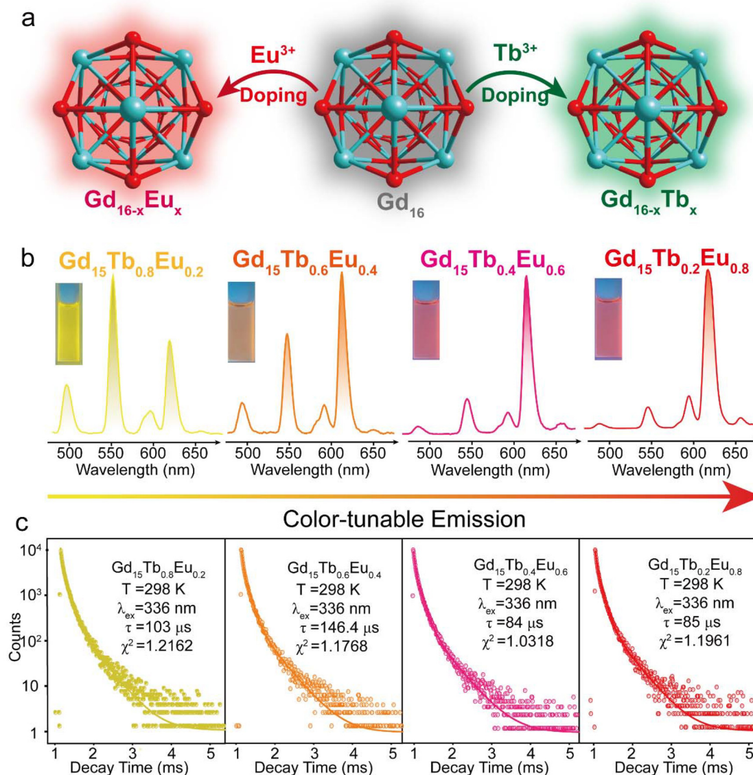
Fig. 3 (a) Schematic illustration of fluorescence colour modulation in \text{Gd}_{16} clusters upon doping with \text{Eu}^{3+} and \text{Tb}^{3+} ions. (b) The emission spectra of \text{Gd}_{15}\text{Tb}_{1-x}\text{Eu}_x ( x = 0.2, 0.4, 0.6, 0.8 ) clusters. (c) The emission decay lifetimes of ^5\text{D}_4 \rightarrow ^7\text{F}_5 transition of \text{Tb}^{3+} at 547 nm in \text{Gd}_{15}\text{Tb}_{1-x}\text{Eu}_x ( x = 0.2, 0.4, 0.6, 0.8 ) clusters.
