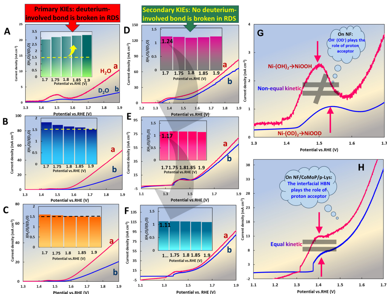
Fig. 6 Kinetic isotopic effect studies. LSVs recorded in \text{H}_2\text{O} (red) and \text{D}_2\text{O} (blue) for the (A) NF, (B) NF/CoMoO 4 , (C) NF/CoMoP, (D) NF/p-Lys, (E) NF/CoMoO 4 /p-Lys and (F) NF/CoMoP/p-Lys electrodes. Comparison of the oxidation peak positions in proteo (red) and deuterio (blue) solutions for \text{Ni}^{2+}/\text{Ni}^{3+} taken for (G) NF and (H) NF/CoMoP/p-Lys, demonstrating the undeniable role of the proton relay groups in the kinetic acceleration of the \text{Ni}(\text{OH})_2/\text{Ni}-\text{OOH} redox couple as a typical PCET reaction.
