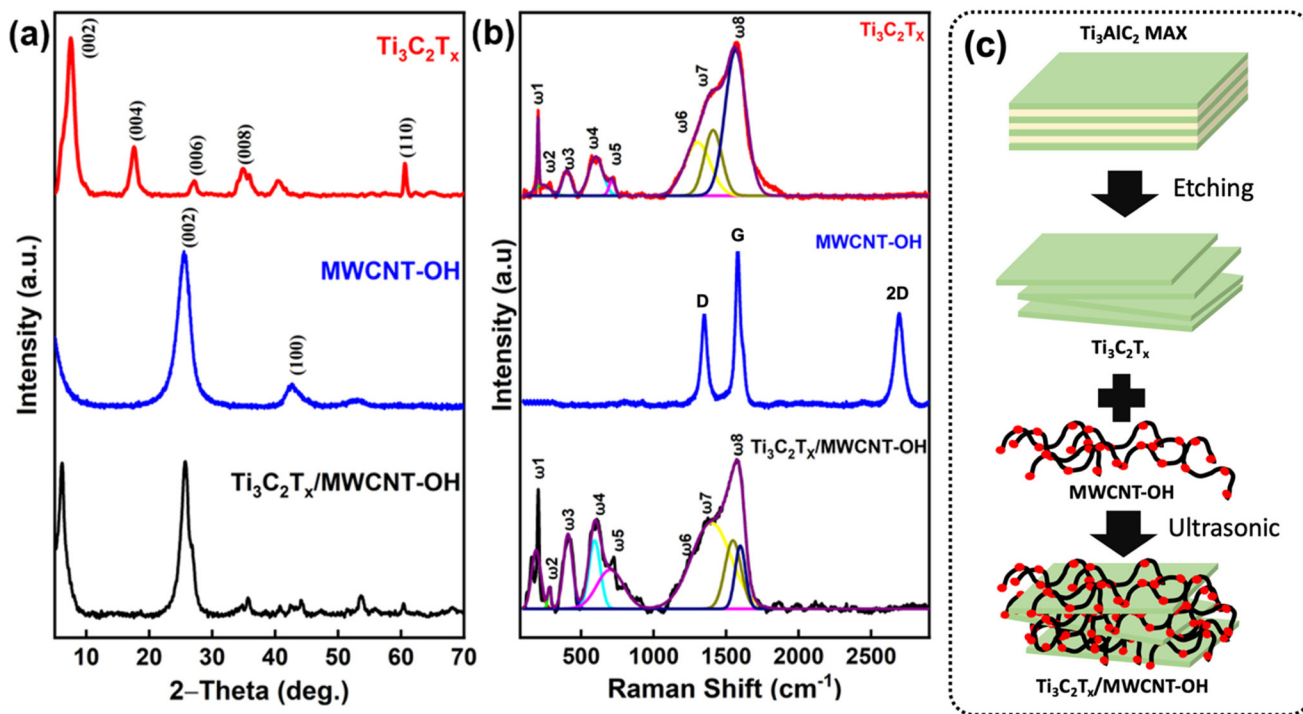
Fig. 1 (a) X-ray diffractogram and (b) Raman spectra of Ti 3 C 2 T x , MWCNT-OH, and Ti 3 C 2 T x /MWCNT-OH nanocomposites; (c) schematic illustration for the formation of nanocomposite.
