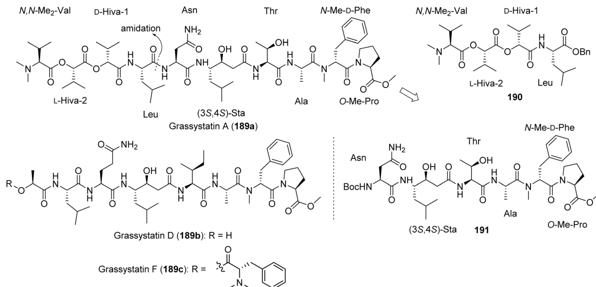
Fig. 46 Chemical structures of grassystatins A ( 189a ), D ( 189b ) and F ( 189c ) with retrosynthetic strategy.
