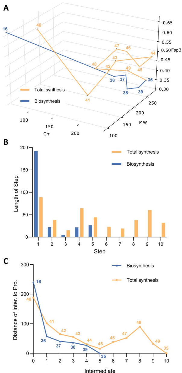
Fig. 3 Chemical space analysis for the production of citrinin 35 . (A) The biosynthesis and chemical synthesis of citrinin 35 illustrated as a C_m , MW and Fsp^3 parameterized 3D plot; (B) bar chart of distance for each step; (C) line chart of distance of each intermediate to final product.
