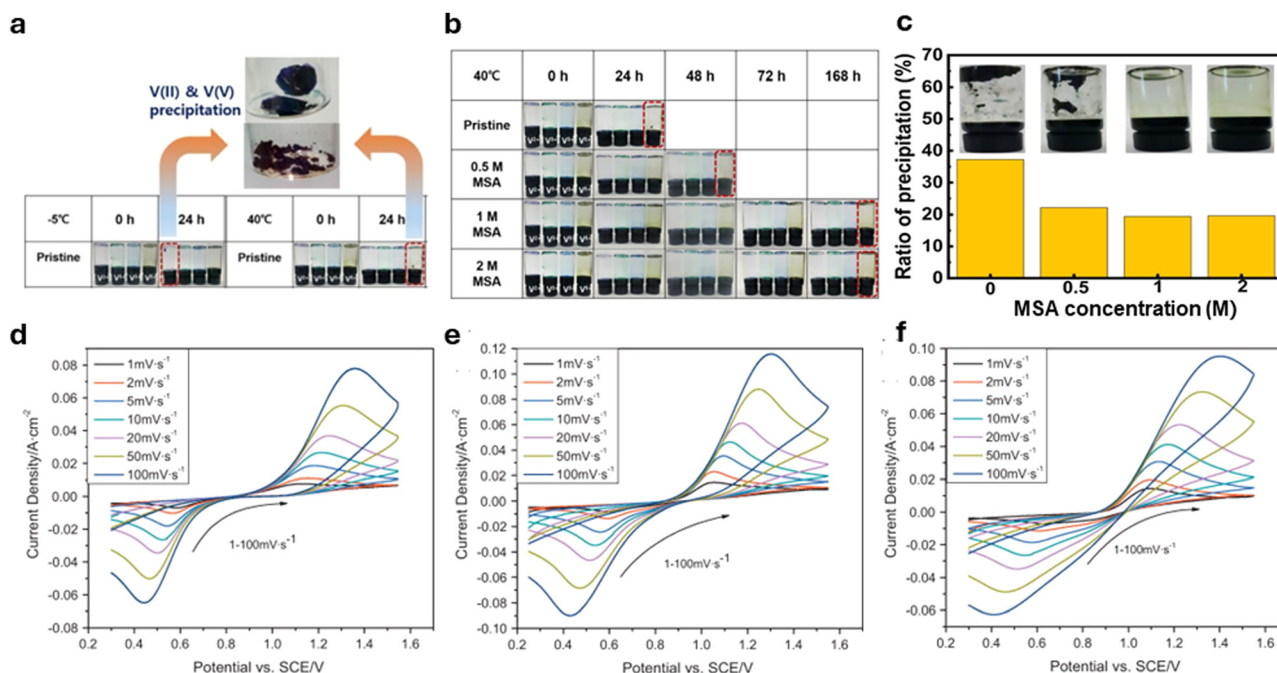
Fig. 14 Schematic of (a) V precipitation without MSA addition at -5 °C and 40 °C at 0 h and 24 h. V precipitation after the stability test of (b) V(II) electrolyte with MSA addition and (c) V(V) electrolyte with MSA addition. 65 Copyright 2021, Elsevier. (d)–(f) Cyclic voltammograms of a stationary Pt electrode in V(V)/V(IV)-MSA solutions with different concentrations of V(V)/V(IV) and scan rates from 1 to 100 mV s -1 . 3 Copyright 2012, Elsevier.
