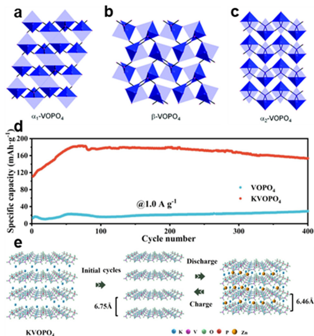
Fig. 9 Schematic of (a)–(c) Structures of vanadium phosphates in \alpha_1 , \alpha_2 and \beta phases. 32 Copyright 2013, the Royal Society of Chemistry. (d) Reversible capacity of the \text{VOPO}_4 and \text{KVOPO}_4 electrodes at 1 \text{ A g}^{-1} . (e) Zn-storage mechanism of the \text{KVOPO}_4 electrode during the cycling process. 33 Copyright 2024, Elsevier.
