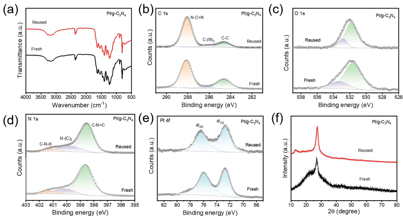
Fig. 5 The characterization of Pt/g-C 3 N 4 after five photocatalytic cycles. (a) FTIR spectra. (b–e) XPS spectra of C 1s (b), O 1s (c), N 1s (d), and Pt 4f (e). (f) XRD patterns.
