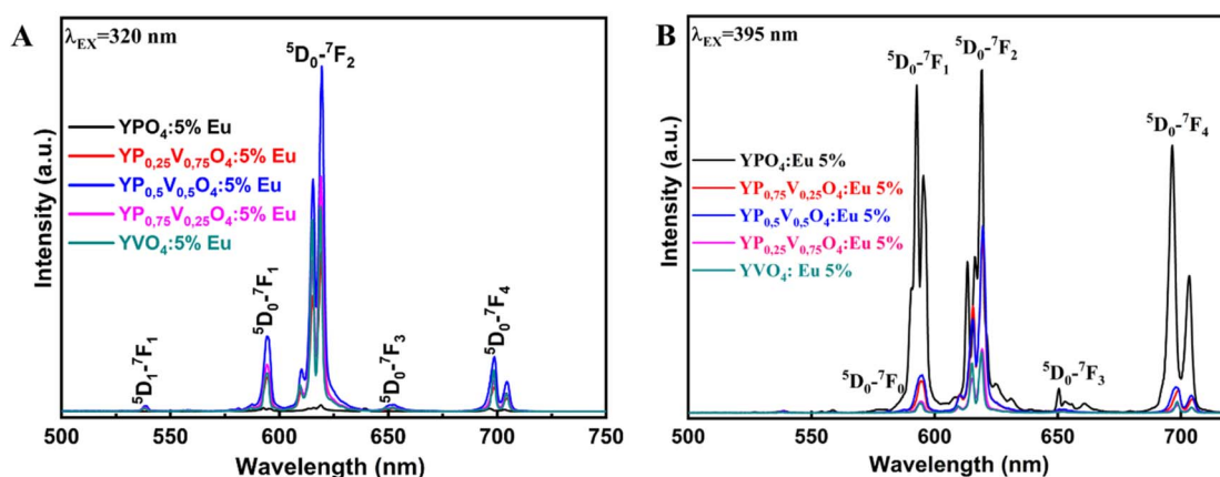
Fig. 7 Fluorescence spectra of Y(P_{1-x}V_x)O_4:5\% \text{ Eu} samples under (A) 320 nm and (B) 395 nm excitation.
