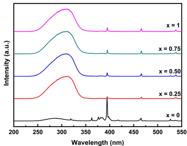
Fig. 5 Fluorescence excitation spectrum of Y(P_{1-x}V_x)O_4:5\% \text{ Eu} materials ( x = 0, 0.25, 0.5, 0.75, and 1 ).
