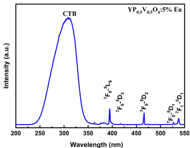
Fig. 6 The fluorescence excitation spectrum of the Y(P_{0.5}V_{0.5})O_4:5\% \text{ Eu} material.
