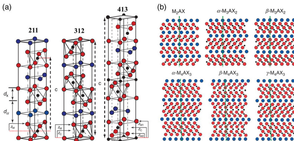
Fig. 3 Crystal structure of 211, 312, and 413 MAX phases. (a) Unit cell of the three phases. The lattice parameter c of each unit cell is outlined by vertical dashed lines. The thicknesses of the M_6X layer and A layer are denoted as d_x and d_a , respectively. (b) Schematics of the [11\bar{2}0] planes and the polymorphism of the MAX phases. Reproduced with permission. 35 Copyright 2020 Wiley-VCH GmbH.
