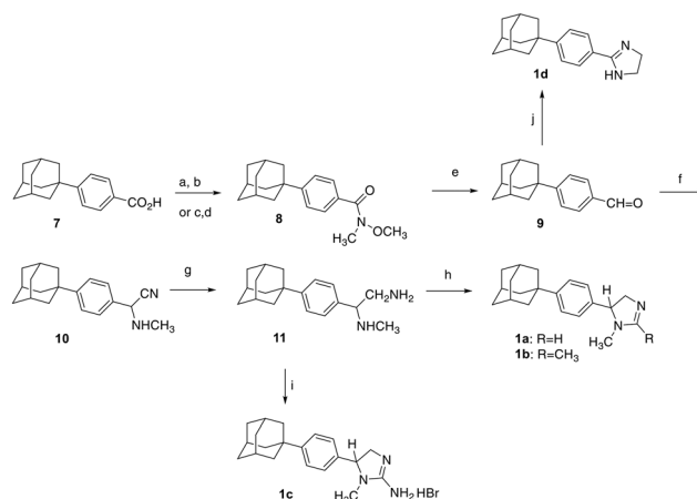
Scheme 1 Reagents and conditions: (a) N(\text{CH}_2\text{CH}_2\text{OMe})_2\text{SF}_3 , DIPEA, DCM, 0 °C, 30 min; (b) \text{HN}(\text{OMe})\text{Me}\cdot\text{HCl} , DIPEA, DCM, 0 °C, 30 min, rt for 24 h, 55 °C for 24 h; (c) \text{PPh}_3 , NBS, 0 °C, 15 min; (d) \text{HN}(\text{OMe})\text{Me}\cdot\text{HCl} , \text{Et}_3\text{N} , DCM, rt, 3 h; (e) LDBBA, THF, 0 °C, 30 min; (f) NaCN, \text{CH}_3\text{NH}_2\cdot\text{HCl} , DMSO : \text{H}_2\text{O} , 9 : 1, 60 °C, 7 h; (g) \text{H}_2/\text{PtO}_2 , EtOH, \text{HCl}(\text{g})/\text{EtOH} , 55 psi, rt, 4.5 h; (h) formamide acetate or acetamide hydrochloride, EtOH, reflux, 48 h; (i) BrCN, DCM, rt, 48 h; (j) \text{I}_2 , ethylenediamine, \text{K}_2\text{CO}_3 , tert -BuOH, 70 °C, 3 h.
