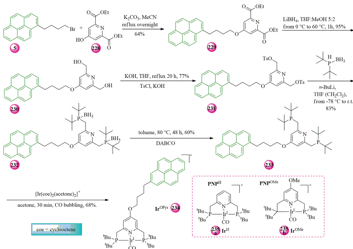
Fig. 67 The synthesis procedure for the ligand \text{PNP}^{\text{OPyr}} ( 233 ) and the schematic structure of \text{Ir}^{\text{H}} ( 235a ) and \text{Ir}^{\text{OMe}} ( 235b ). Reproduced with permission from ref. 76 copyright 2023, John Wiley and Sons.
