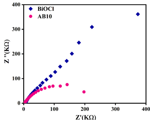
Fig. 7 EIS Nyquist plot of BiOCl and AB10.
