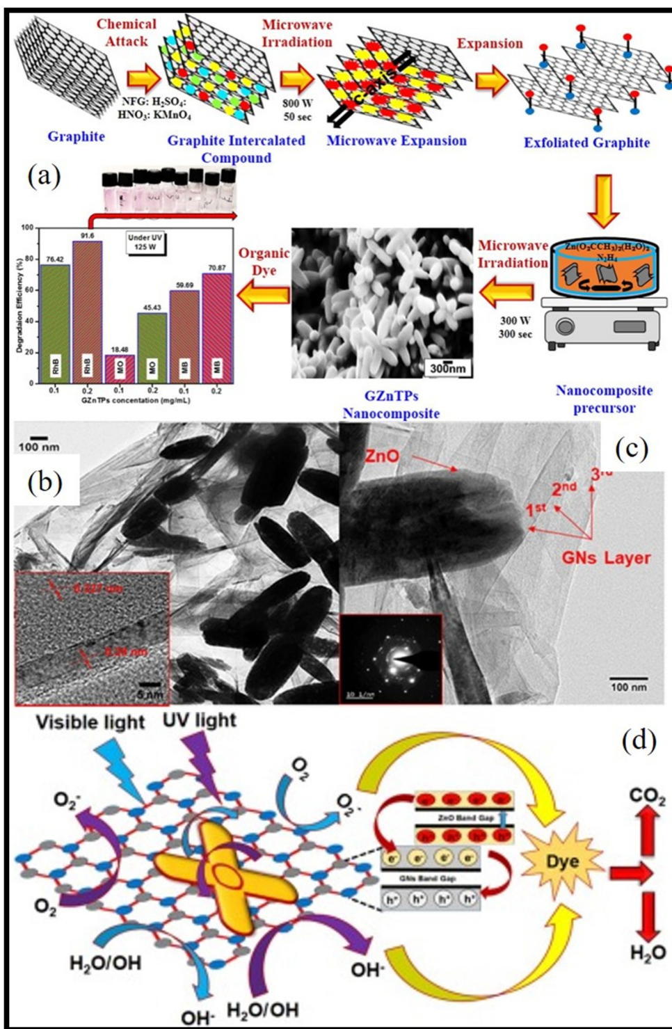
Fig. 11 GNs-ZnO TPs nanocomposites: (a) schematic of synthesis of GNs-ZnO TPs nanocomposites by microwave synthesis including SEM image of nanocomposites (b) and (c) HRTEM and (d) photocatalytic mechanism of GNs-ZnO TPs nanocomposites. [Reprinted with permission from ref. 84 Copyright 2021, Elsevier].
