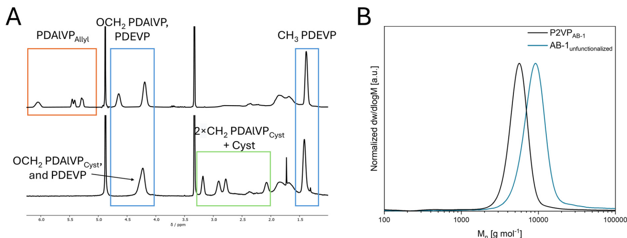
Fig. 1 (A) ^1\text{H} -NMR spectra showing successful and quantitative thiol–ene functionalization of \text{ABB}'\text{-}2_{\text{Allyl}} (A, top), resulting in \text{ABB}'\text{-}2_{\text{Cyst}} (A, bottom). Blue: Aliphatic side-chain protons of phosphorus-containing monomer units. Orange: Allylic protons of PDAIVP. Green: \text{CH}_2 protons of the former allyl group and cysteamine protons incorporated into \text{ABB}'\text{-}2_{\text{Cyst}} (B) SEC traces of block A (black) and AB (blue) of block copolymer AB-1 showing successful block copolymer formation indicated by a shift of the signal towards higher molar masses.
