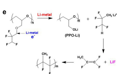
Fig. 3 Mechanism of solvent-derived fluorinated SEIs. (a) Non-fluorinated SEI derived from EC/EMC-based solvent vs. fluorinated SEI derived from FEC/EMC based solvent. Reproduced with permission. 37 Copyright 2018, American Chemical Society; (b) schematic illustration of desolvation mechanisms in p(PEE-DOL). Reproduced with permission. 40 Copyright 2023, Elsevier; (c) molecular design of DFA with inert methoxyl and AFA with an active nitrate ending group on the side of the fluorocarbon segment. Reproduced with permission. 41 Copyright 2022, John Wiley and Sons; (d) reaction mechanism of in situ formation of LiF by the PF monomer in the MG-PF-PU polymer. Reproduced with permission. 42 Copyright 2024, John Wiley and Sons; (e) reaction mechanism of TFP-containing polymers with Li-metal. Reproduced with permission. 43 Copyright 2022, John Wiley and Sons; (f) reaction mechanism of C5-POE-F with Li-metal. Reproduced with permission. 44 Copyright 2021, John Wiley and Sons.
