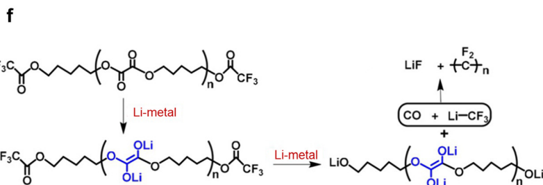
Fig. 3 Mechanism of solvent-derived fluorinated SEIs. (a) Non-fluorinated SEI derived from EC/EMC-based solvent vs. fluorinated SEI derived from FEC/EMC based solvent. Reproduced with permission. 37 Copyright 2018, American Chemical Society; (b) schematic illustration of desolvation mechanisms in p(PEE-DOL). Reproduced with permission. 40 Copyright 2023, Elsevier; (c) molecular design of DFA with inert methoxyl and AFA with an active nitrate ending group on the side of the fluorocarbon segment. Reproduced with permission. 41 Copyright 2022, John Wiley and Sons; (d) reaction mechanism of in situ formation of LiF by the PF monomer in the MG-PF-PU polymer. Reproduced with permission. 42 Copyright 2024, John Wiley and Sons; (e) reaction mechanism of TFP-containing polymers with Li-metal. Reproduced with permission. 43 Copyright 2022, John Wiley and Sons; (f) reaction mechanism of C5-POE-F with Li-metal. Reproduced with permission. 44 Copyright 2021, John Wiley and Sons.
