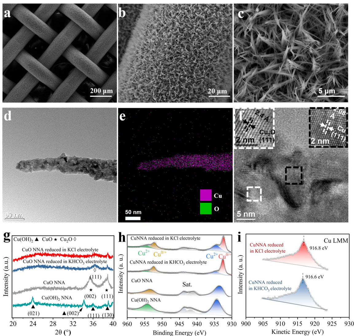
Fig. 1 (a–c) SEM images of the Cu NNA catalyst; (d) TEM images, (e) elemental mapping, (f) high resolution TEM of the Cu NNA catalyst after \text{CO}_2\text{RR} in \text{KHCO}_3 electrolyte; (g) XRD spectrogram, (h) XPS spectrogram of Cu 2p spectrogram for \text{Cu}(\text{OH})_2 , Cu NNA, and CuNNA after in situ reduction; (i) Cu LMM spectrogram of the Cu NNA catalyst reduced in KCl and \text{KHCO}_3 electrolytes.
