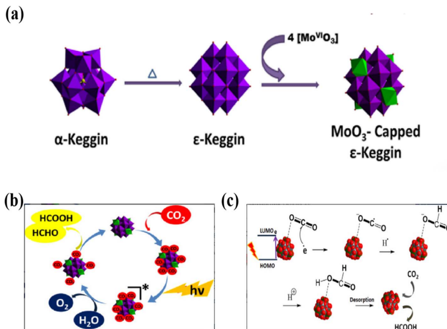
Fig. 2 (a) Possible formation pathway of the \{\text{Mo}16\} unit; (b) proposed plausible mechanism for \text{CO}_2 photoreduction; (c) schematic diagram showing a proposed mechanism for the reduction of \text{CO}_2 to formic acid. 84
