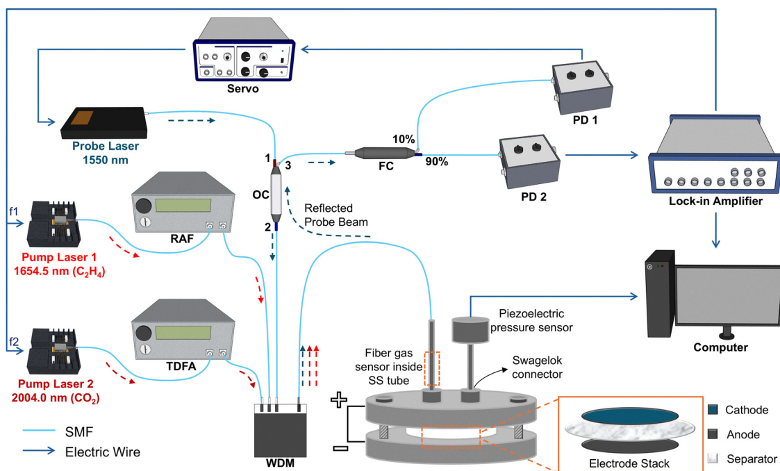
Fig. 3 HCF-PTS gas sensing platform for Li-ion cells. The experimental setup for simultaneous detection of \text{C}_2\text{H}_4 and \text{CO}_2 . f_1 = 10 \text{ kHz} and f_2 = 8 \text{ kHz} are the modulation frequencies for pump laser 1 (for \text{C}_2\text{H}_4 ) and 2 (for \text{CO}_2 ). RFA: Raman fiber amplifier. TDFA: Thulium-doped fiber amplifier. OC: optical circulator. PD: photodetector. WDM: wavelength-division multiplexing. FC: fiber coupler. LIA: lock-in amplifier. A two-channel LIA is used for simultaneous detection of \text{C}_2\text{H}_4 and \text{CO}_2 . The schematic of the homemade cell is also provided with the electrode stack being illustrated. Although the customized interrogation system in a lab scale may look bulky, it can be integrated into circuit boards to achieve the size of a desktop computer for application purposes. The digital images of the necessary components are supplied in Note 1, SI.
