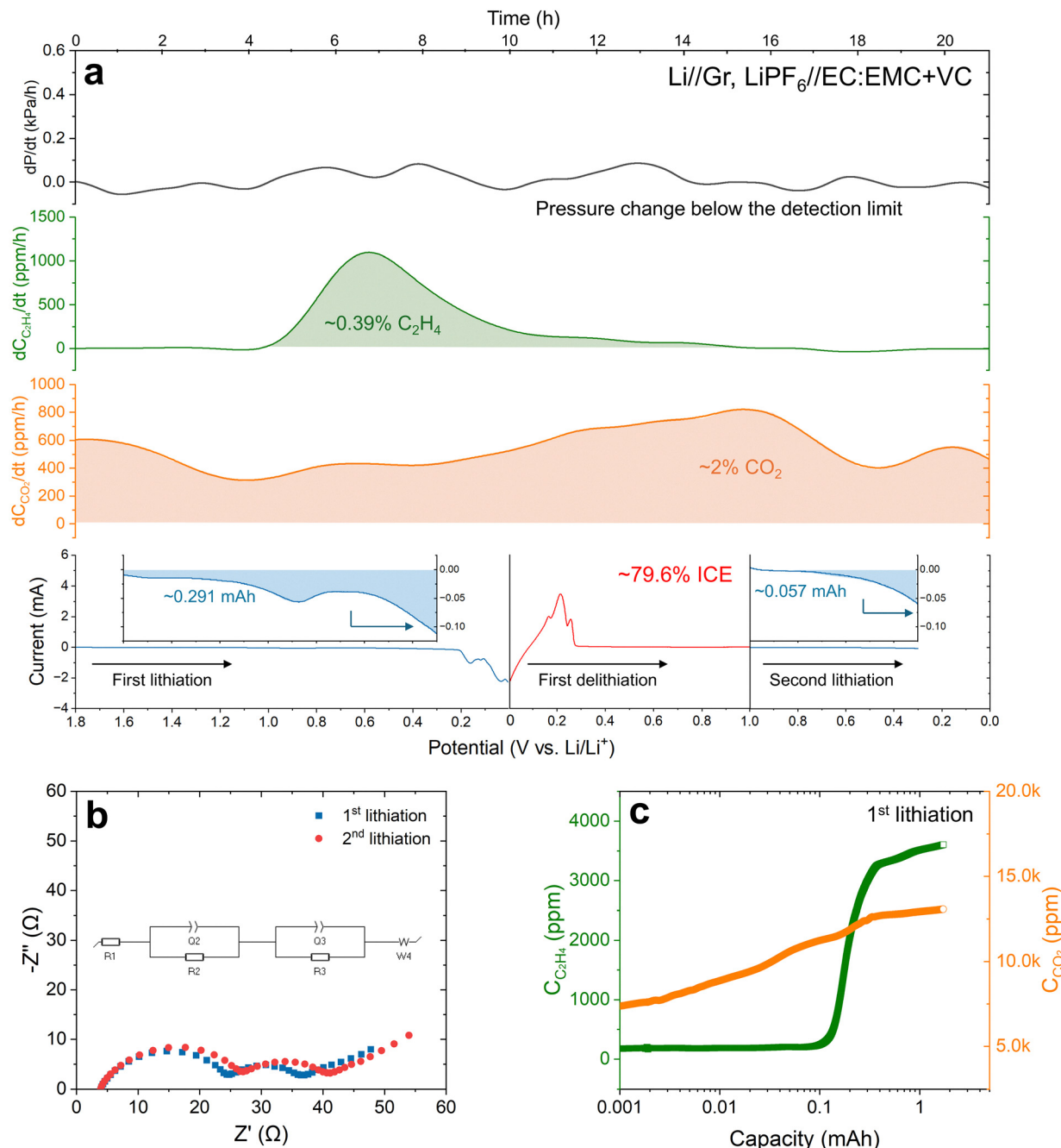
Fig. 7 Operando monitoring of gas evolution in the Li-graphite half-cell that undergoes cyclic voltammetry at a scan rate of 0.05 \text{ mV s}^{-1} with 1 M \text{LiPF}_6 in EC : EMC 3 : 7 vol% + 2 vol% VC as the electrolyte. (a) The obtained CV curves are plotted in conjunction with the change in concentrations of \text{C}_2\text{H}_4 , \text{CO}_2 , and in overall gas pressure. The detailed current variation from 1.8 V to 0.3 V vs. \text{Li/Li}^+ of the first lithiation and from 1.0 V to 0.3 V vs. \text{Li/Li}^+ of the second lithiation is provided in the insets by zooming in the y-axis. The blue shading of the first lithiation represents the electric charge consumed for the SEI formation and associated gas evolution. (b) The EIS spectra obtained after the initial and the second cathodic scan. (c) Evolution of \text{C}_2\text{H}_4 and \text{CO}_2 concentrations during the initial lithiation of graphite.
