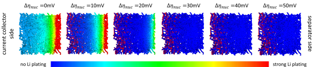
Fig. 6 Top: influence of a gradient in lithiophilicity on the ratio of the effective, mean amount of Li plating on the current collector and separator sides of different porous microstructures (train 11 635, train 5481, and train 44 842; cf. Table S3†) with similar thickness and similar capacity after 10 s at 0.1 \text{ mA cm}^{-2} . An extended figure which additionally includes a dual-layer structure with a surface area and porosity gradient can be found in the ESI (Fig. S19†). Bottom: the amount of plated Li on a highly porous (90%) fiber system with different lithiophilicity (train 11 635; cf. Table S3†) in combination with a thin lithiophilic interlayer ( \eta_{\text{nuc}} = 0 \text{ V} ) after 10 s at 0.1 \text{ mA cm}^{-2} . The shown view is from the side in the through direction. The current collector is located on the left side, while the separator is beginning on the right. An extended figure including all three structures with different porosities can be found in the ESI (Fig. S18†).
