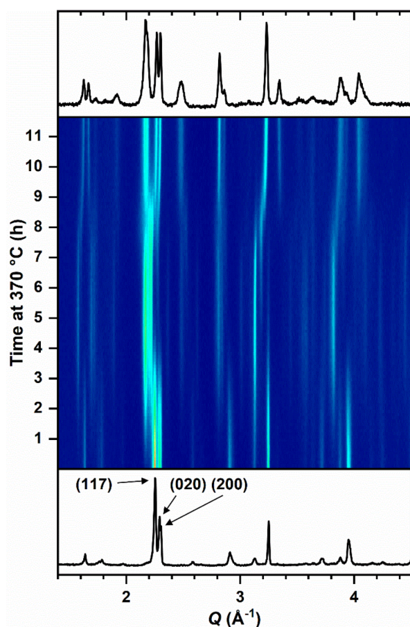
Fig. 2 Time dependent in situ XRD patterns of the reaction of \text{La}_4\text{Ni}_3\text{O}_{10} with PVDF (molar ratio: 1 : 2) obtained at 370 °C. Bottom and top diffraction patterns are the initial and final patterns.
