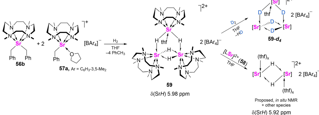
Scheme 22 Synthesis of trinuclear strontium hydride 59 , isotopic exchange with D_2 , and proposed formation of dimeric [L_2Sr_2H_2]^{2+} species in solution.
