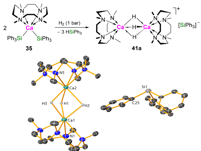
Scheme 10 Hydrogenolysis of compound 35 and molecular structure of dicalcium trihydride silyl complex 41a .
