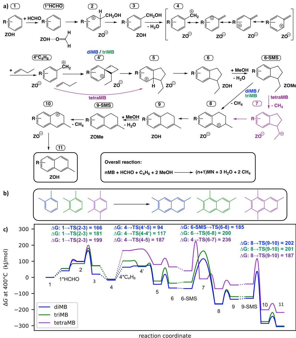
Fig. 2 a) Reaction scheme of the investigated naphthalene formation mechanism. –R = dimethyl, trimethyl, tetramethyl. n MB = n -methylbenzene, ( n + 1). MN = ( n + 1)-methyl-naphthalene. b) Investigated isomers of reactants and products. c) Gibbs free energy diagrams of reaction free energies for naphthalene formation with di-, tri- and tetramethylbenzene. Reaction barrier heights are indicated above the respective barriers. Reaction temperature is 400 °C; reference pressure = 1 bar.
