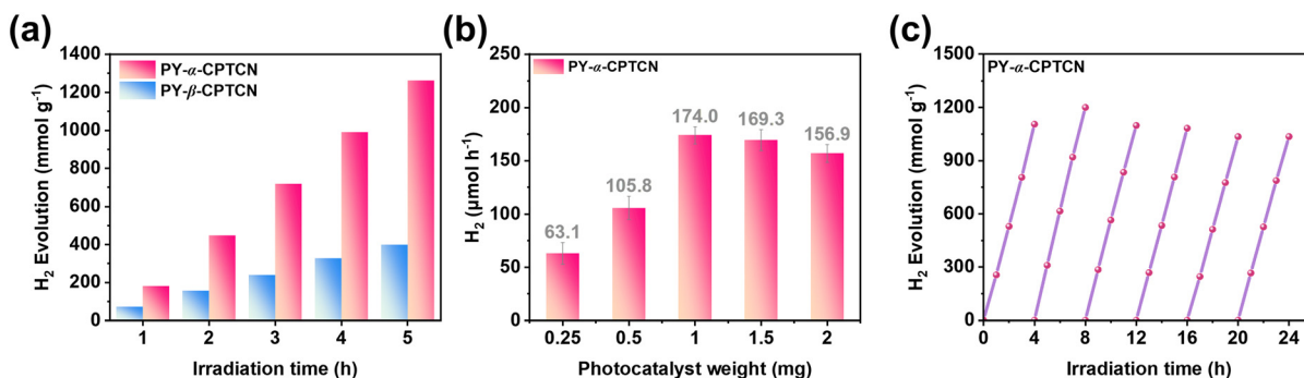
Fig. 2 (a) Hydrogen evolution versus time of PY- \alpha -CPTCN and PY- \beta -CPTCN NPs at the concentration of 5 \mu\text{g mL}^{-1} , under AM 1.5G (100 mW cm -2 ). (b) Photocatalytic \text{H}_2 evolution patterns of PY- \alpha -CPTCN NPs with different weights of the photocatalyst. (c) Time course hydrogen evolution curve of PY- \alpha -CPTCN NPs.
