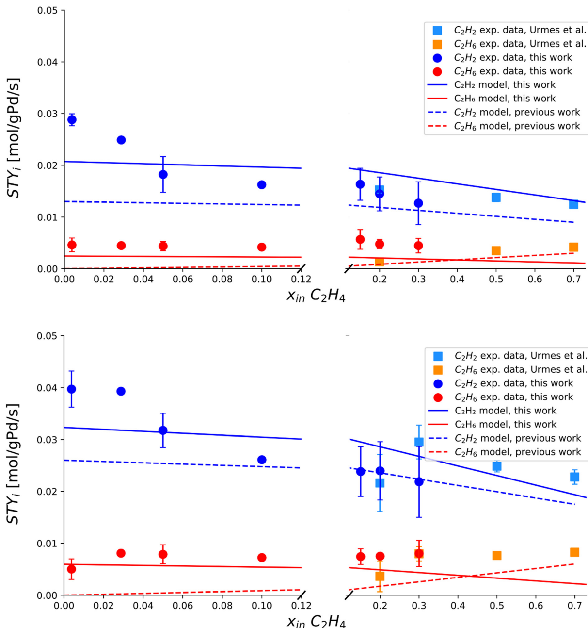
Fig. 7 Experimentally measured and modelled space-time yields of C_2H_2 and C_2H_6 ( STY_{C_2H_2} [ \text{mol gPd}^{-1} \text{s}^{-1} ] and STY_{C_2H_6} [ \text{mol gPd}^{-1} \text{s}^{-1} ]) plotted against the inlet molar fraction of C_2H_4 . Top) Trend obtained at 323 K, i.e. 50 °C. Bottom) Trends obtained at 333 K, i.e. 60 °C. The x-axis is reported with a broken plot representation to precisely quantify the behavior across the composition range investigated. Includes experimental data by Urmès et al., experimental data from this work, model simulation results by this work and a dotted line showing model simulation results by Urmès et al. 11 The standard deviation of experimental measurements is reported through error bars for points whose reproducibility has been verified through at least two repeated experiments.
